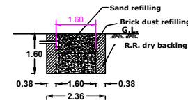
DETAILS OF RAIN WATER HARVESTING Dwg:1A
