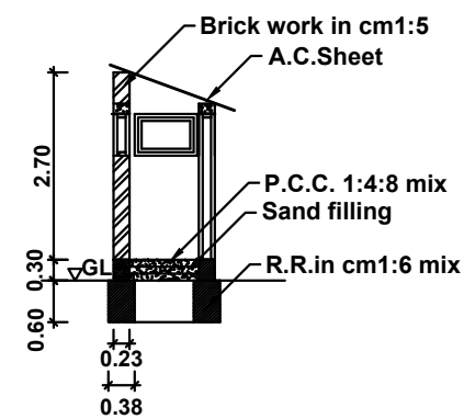
SECTION ON ST
