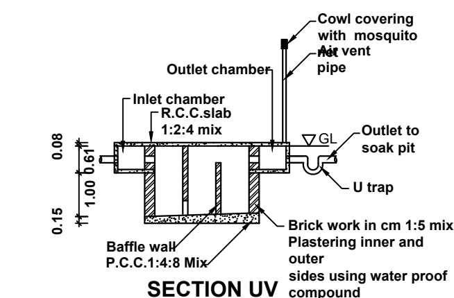
SECTION UV
