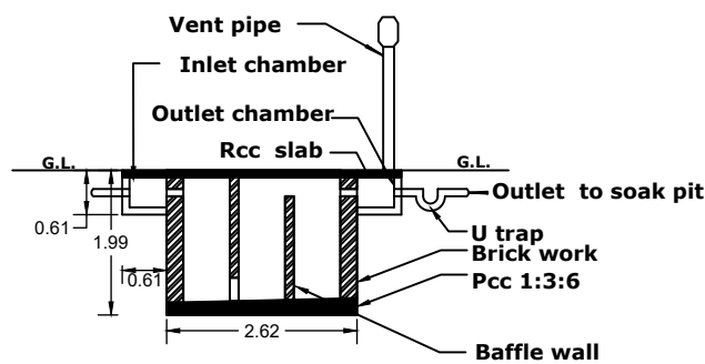
SECTION ON SR
