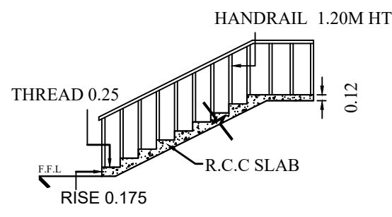
STAIRCASE DETAILS
