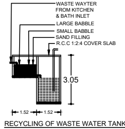
RECYCLING OF WASTE WATER TANK
