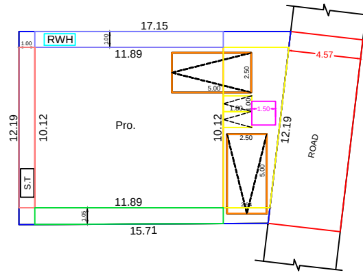
SCALE 1:100
