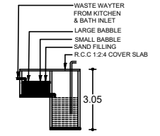
RECYCLING OF WASTE WATER TANK
