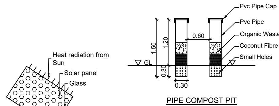
PIPE COMPOST PIT
