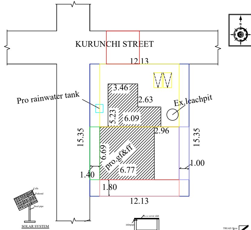
SOLAR SYSTEM
