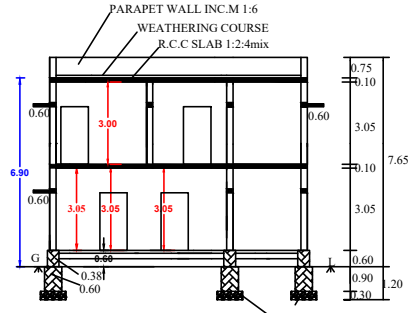
SECTION ON "AB" R.r.masonry in c.m.1:6
