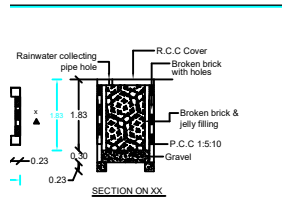
RAINWATER HARVEST WELL
