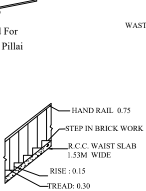
STAIR CASE SECTION
