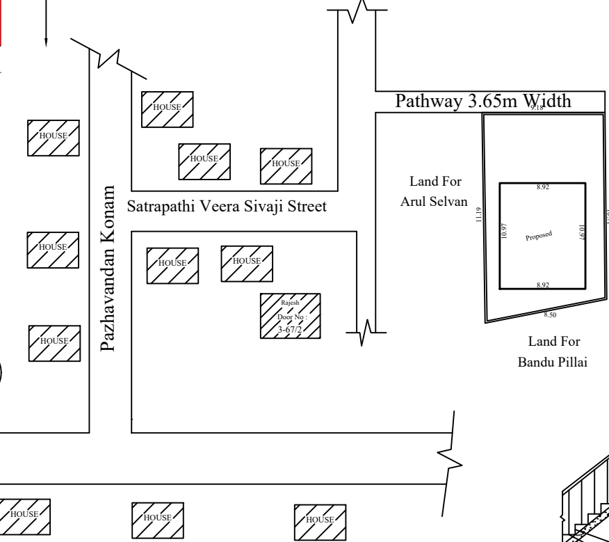
TOPO PLAN
