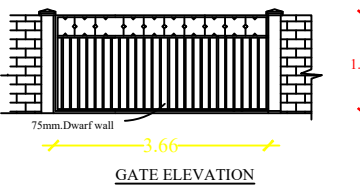
GATE ELEVATION
