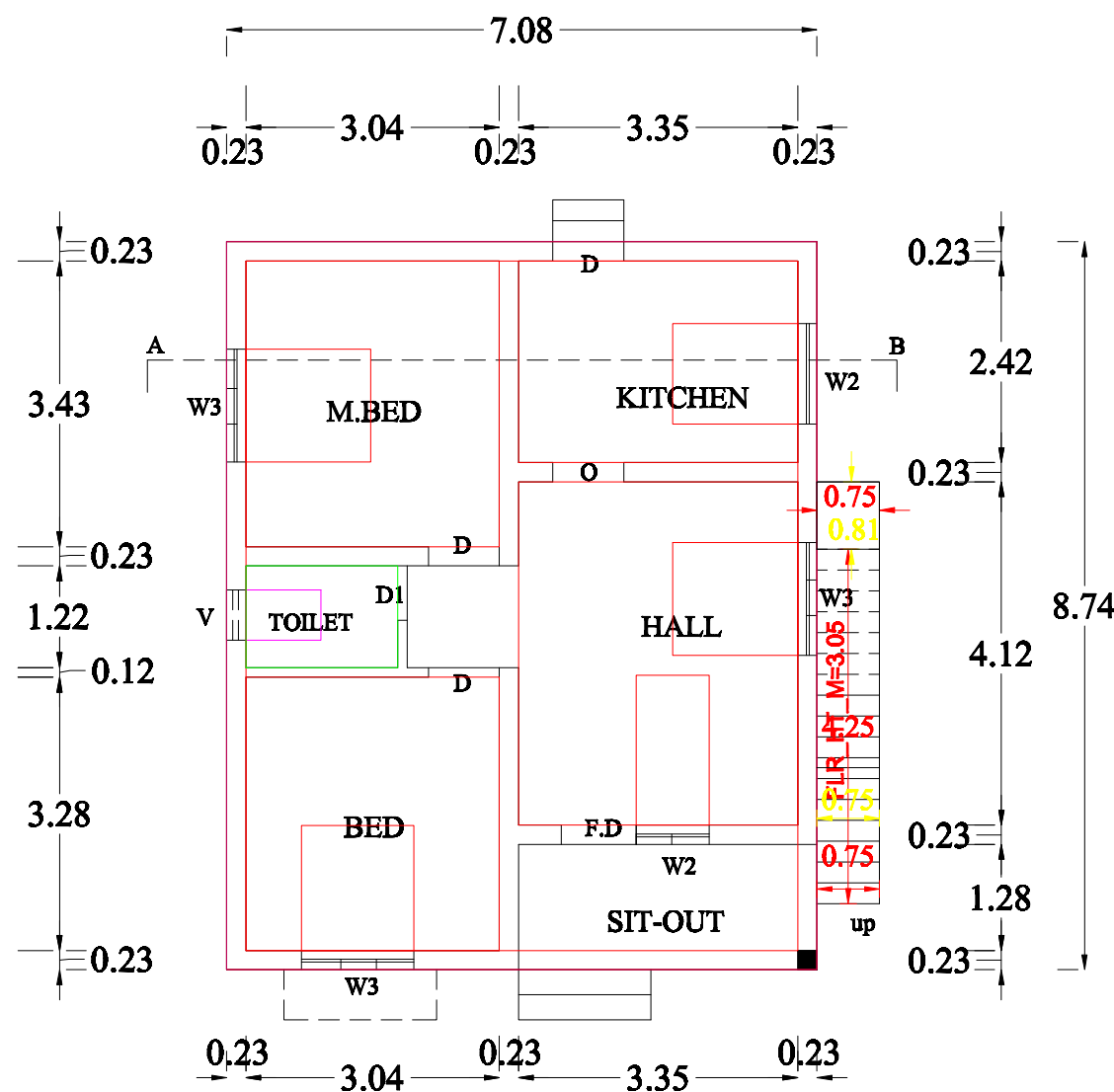
PLAN
