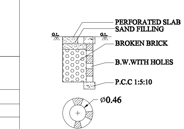
RAIN WATER PERCOLATION DRAWING TYPE -1A
