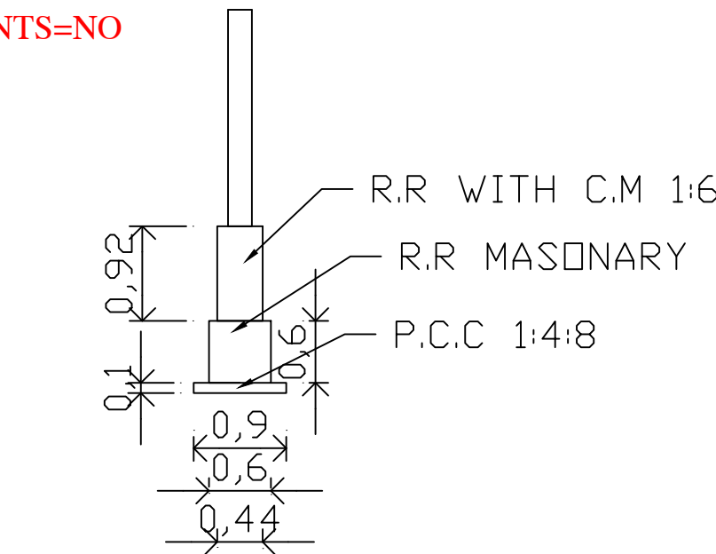
FOUNDATION
