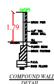
COMPOUND WALL DETAIL
