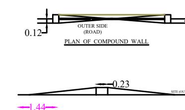
PLAN OF COMPOUND WALL
