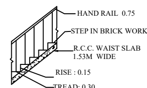
STAIR CASE SECTION
