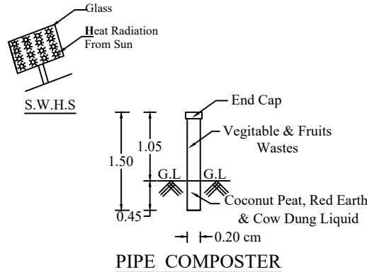
PIPE COMPOSTER
