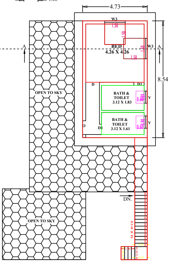
PROPOSED PLAN (FIRST FLOOR)
