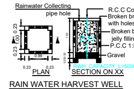
RAIN WATER HARVEST WELL
