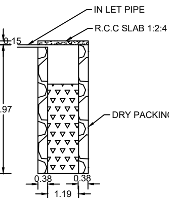
WASTE WATER TANK
