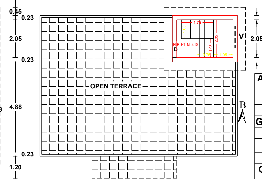
FIRST FLOOR PLAN (HEAD ROOM)
