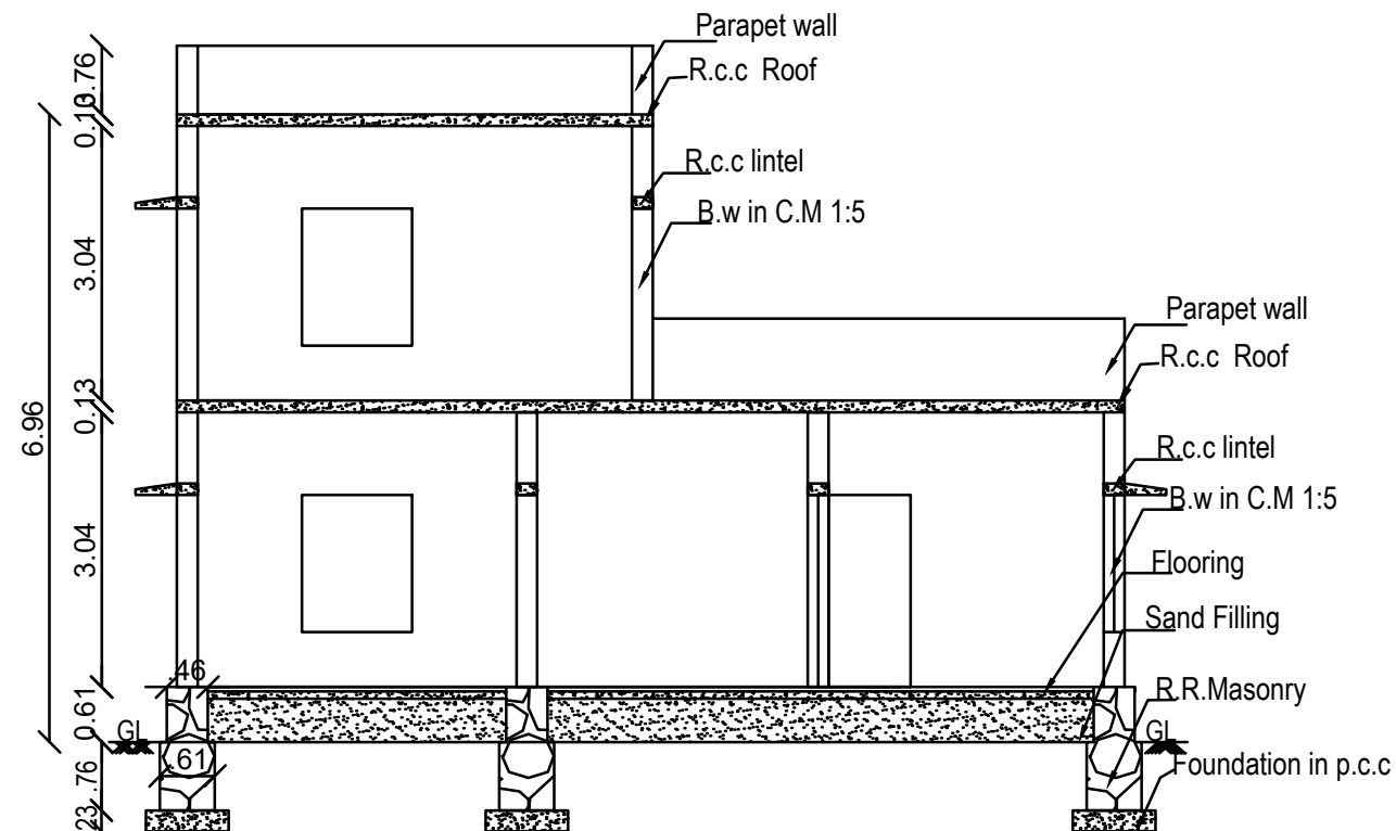
SECTION A&B
