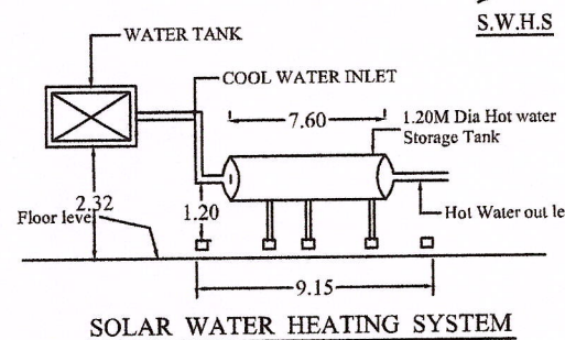
SOLAR WATER HEATING SYSTEM ( S.W.H.S.DETAILS)
