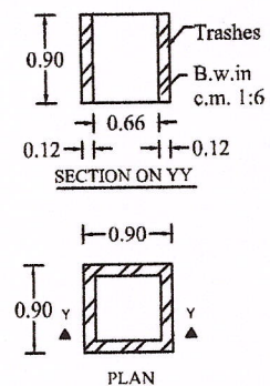
WASTE TRASH PIT
