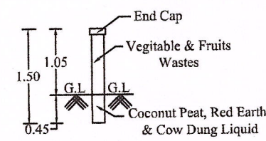
PIPE COMPOSTER
