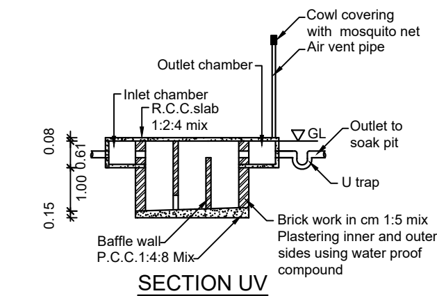
SECTION UV
