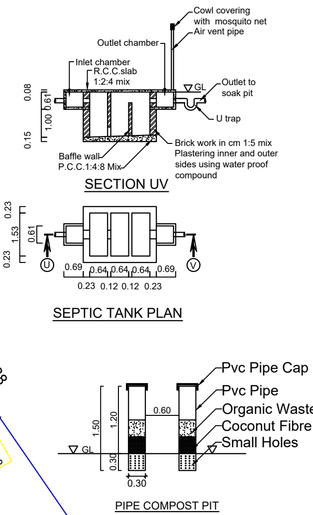
PIPE COMPOST PIT
