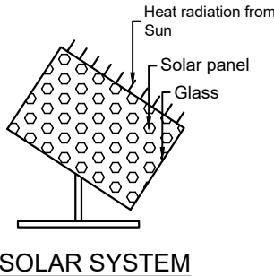
SOLAR SYSTEM
