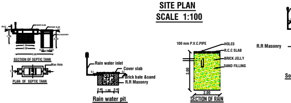
WATER COLLECTING TANK
