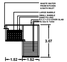
RECYCLING OF WASTE WATER FROM KITCHEN & BATHROOM
