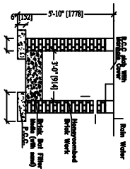
SECTION X-X
