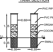
PIPE COMPOSITE PIT
