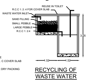
RECYCLING OF WASTE WATER
