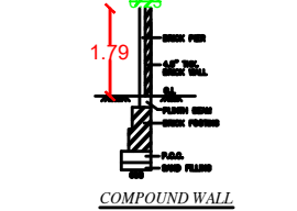
COMPOUND WALL DETAIL
