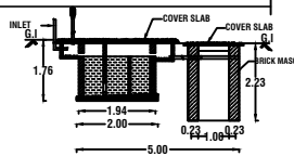
SECTION OF SEPTIC TANK
