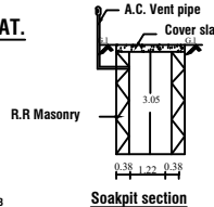
Soakpit section
