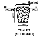
TRIAL PIT (NOT TO SCALE)
