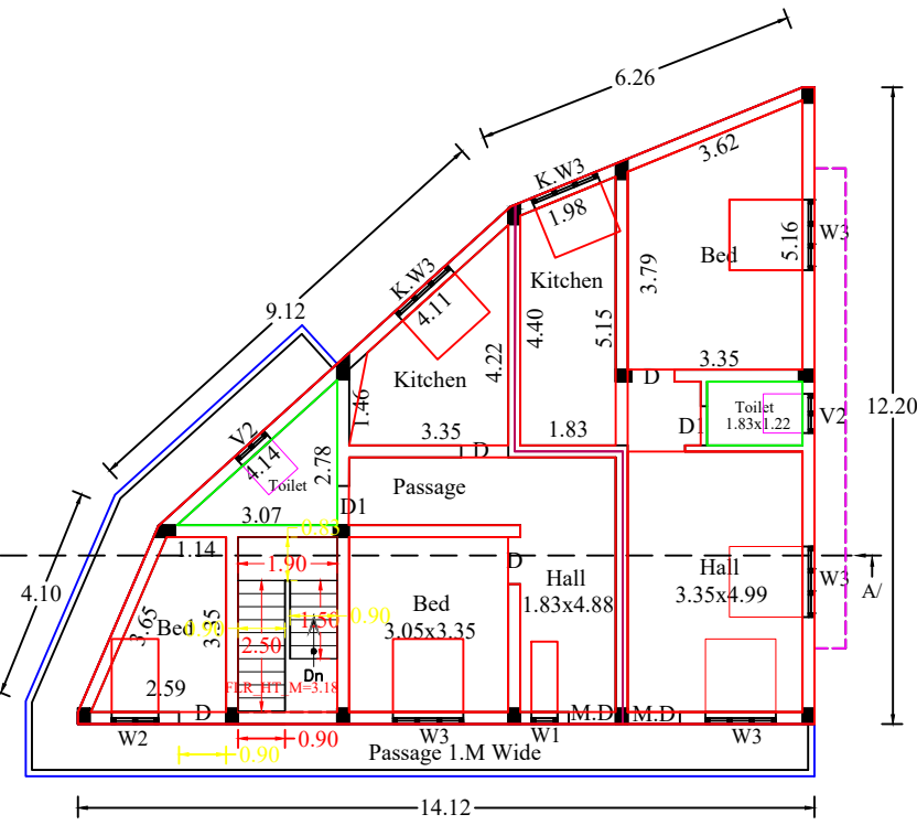
EXTENSION FIRST FLOOR PLAN
