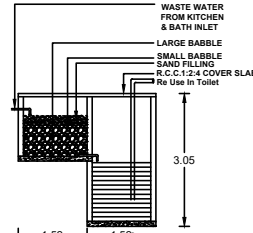
RECYCLING OF WASTE WATER FROM BATHROOM & KITCHEN
