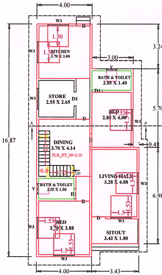
PLAN (GROUND FLOOR)
