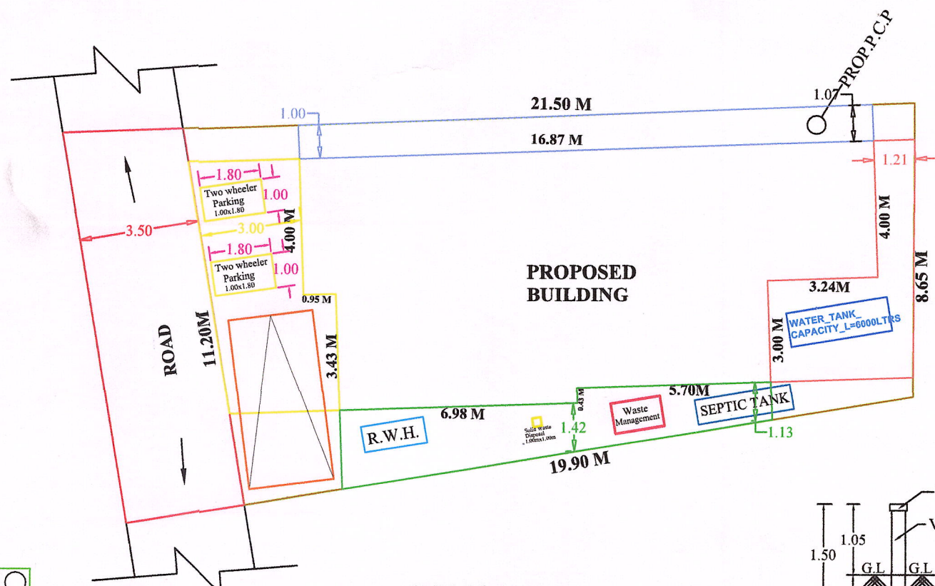
SITE PLAN
