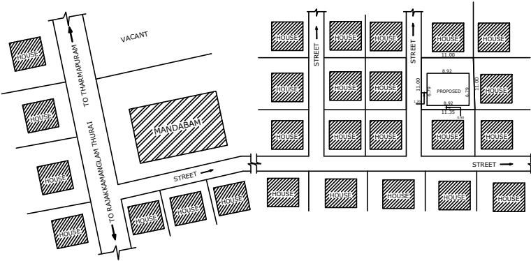
KEY PLAN [SCALE 1:400]
