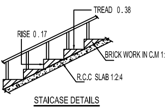
STAIRCASE DETAILS
