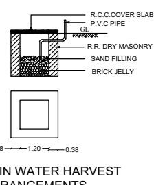
RAIN WATER HARVEST ARRANGEMENTS
