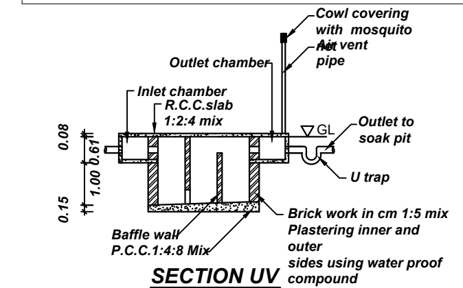
SECTION UV
