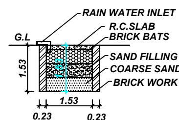
RAIN WATER HARVESTING PIT RWH_CAPACITY_L=5000LTRS
