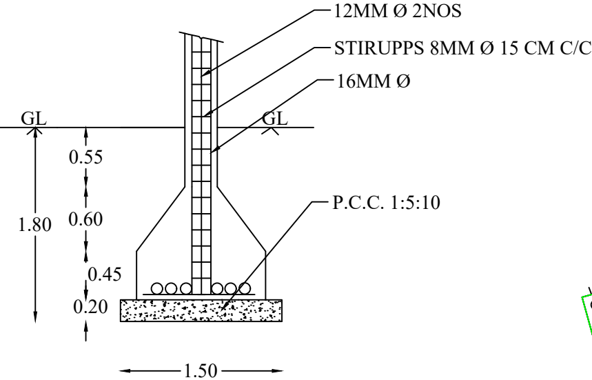
COLUMN DETAILS (SIZE 0.23X0.30)
