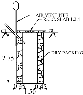
SOAK PIT DETAILS
