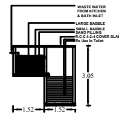
RECYCLING OF WASTE WATER FROM KITCHEN & BATHROOM
