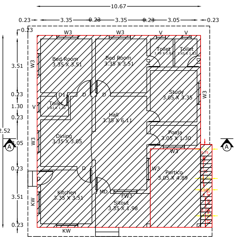
EX. GROUND FLOOR PLAN
