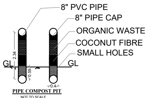
PIPE COMPOST PIT NOT TO SCALE
