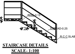
STAIRCASE DETAILS SCALE- 1:100
