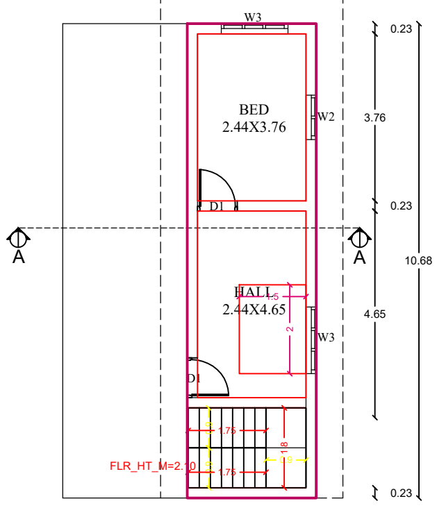
FIRST FLOOR PLAN (PROPOSED) Area = 30.97 Sq.M (333.24 Sq.Ft)
