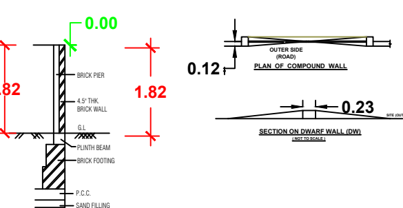
COMPOUND WALL
