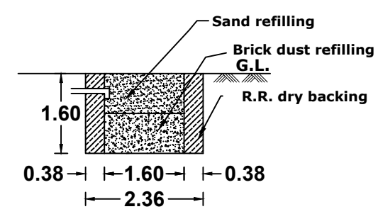
DETAILS OF RAIN WATER HARVESTING
