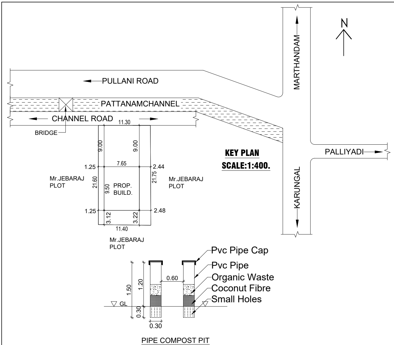
PIPE COMPOST PIT
