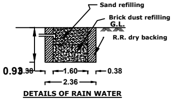
DETAILS OF RAIN WATER
