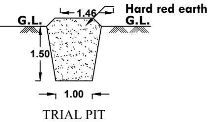
TRIAL PIT
