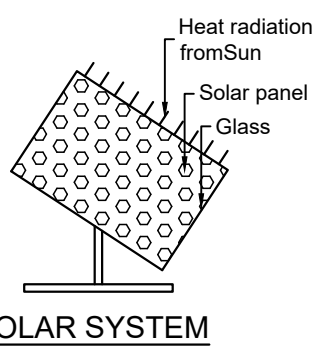
SOLAR SYSTEM
