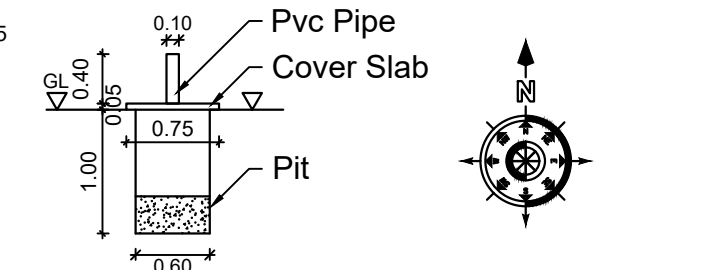
SOLID WASTE COMPOST PIT
