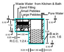
WASTE WATER RECYCLING SYSTEM
