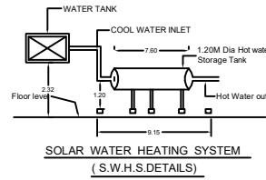
SOLAR WATER HEATING SYSTEM (S.W.H.S.DETAILS)
