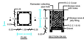
RAIN WATER HARVEST WELL
