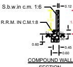
COMPOUND WALL SECTION
