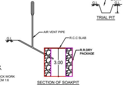
SECTION OF SOAKPIT
