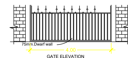
GATE ELEVATION
