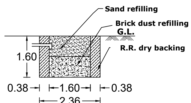
DETAILS OF RAIN WATER HARVESTING
