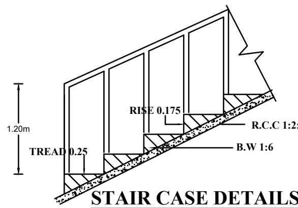
STAIR CASE DETAILS
