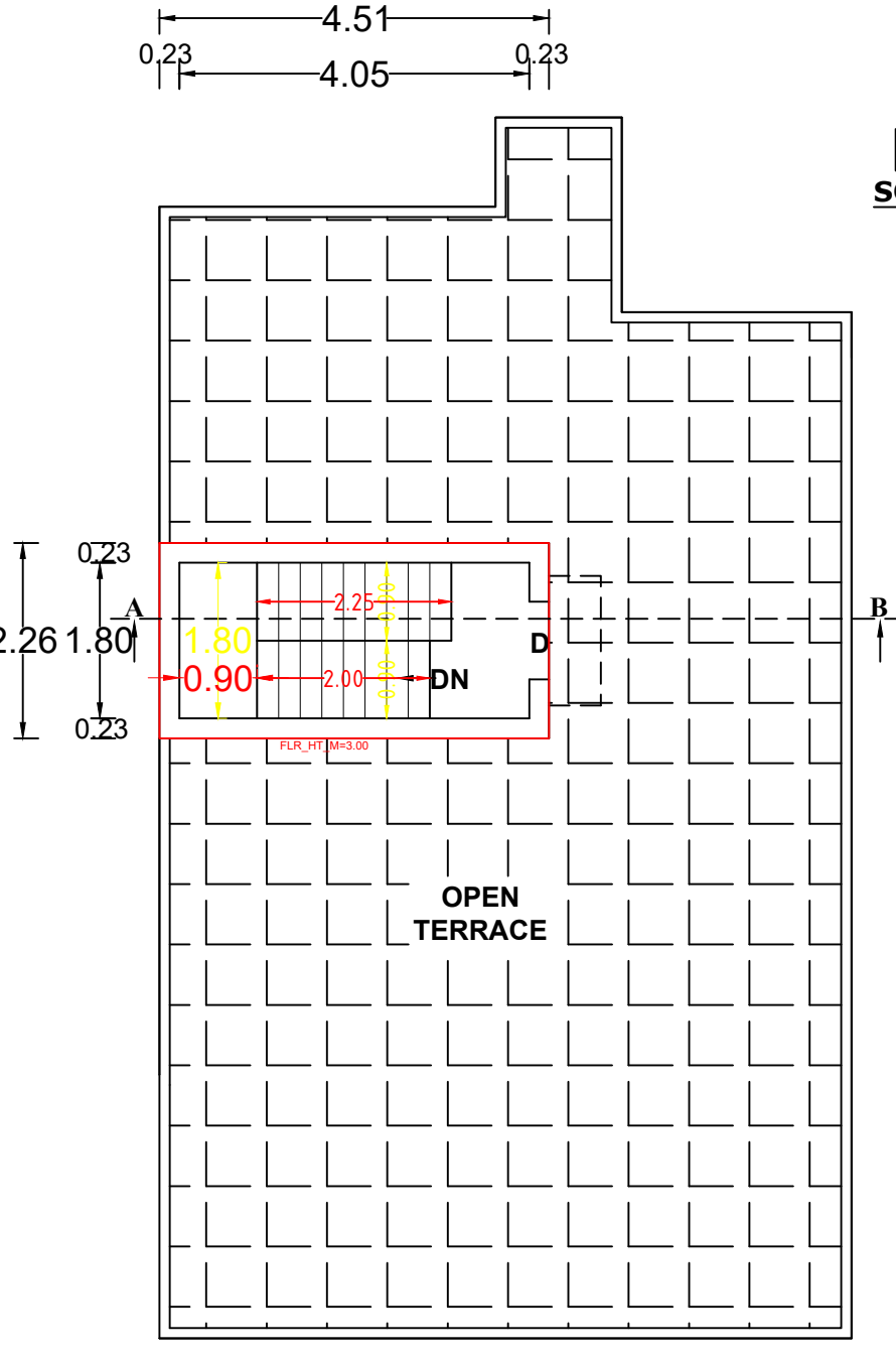
HEAD ROOM PLAN
