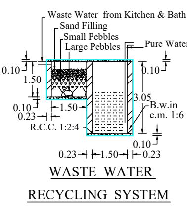
WASTE WATER RECYCLING SYSTEM
