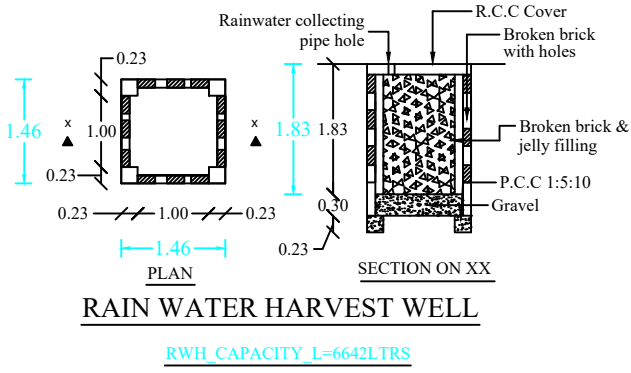
RWH CAPACITY L=6642LTRS
