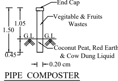
PIPE COMPOSTER
