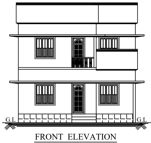
FRONT ELEVATION
