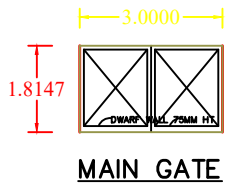
MAIN GATE
