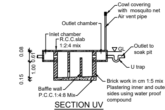
SECTION UV
