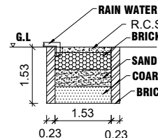
RAIN WATER HARVESTING PIT
