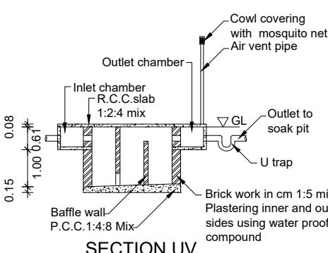
SECTION UV
