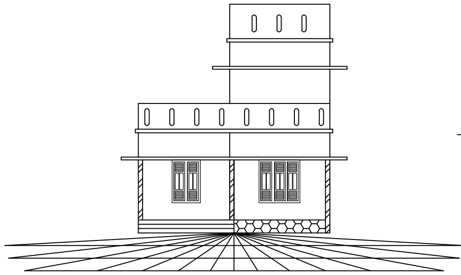
ELEVATION SCALE- 1:100
