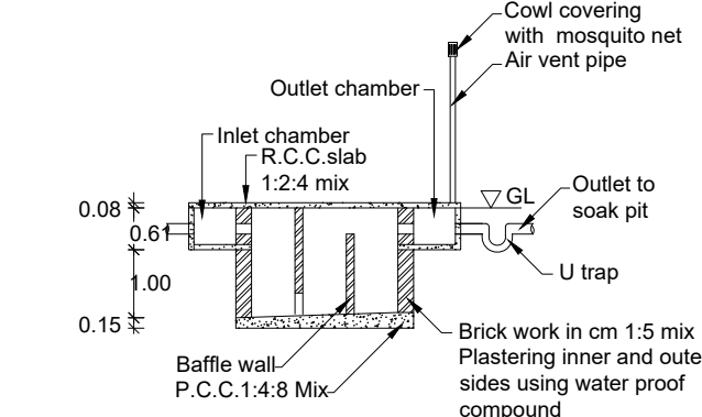
SECTION UV
