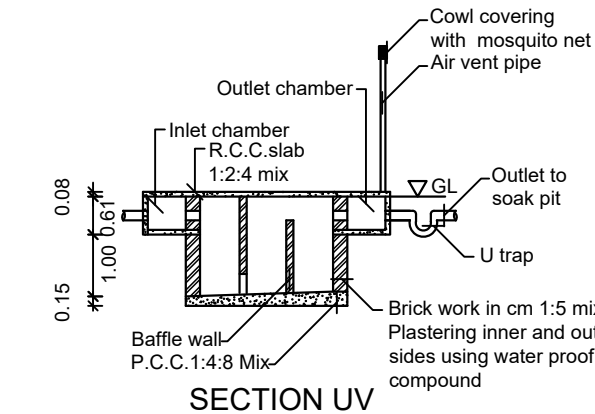
SECTION UV
